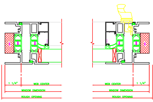
430 JAMB 325 CASEMENT IN 4-BAR ARMS
