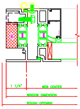
432 JAMB 325 CASEMENT IN BUTT HINGES
